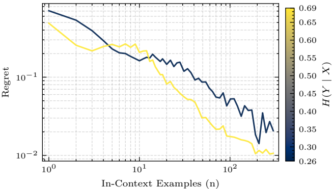
In-Context Learning Regret for Qwen-2.5 (14B)
